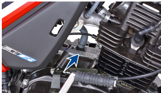
Engine serial number is stamped on the top surface of the left side crankcase assembly near cylinder block.
